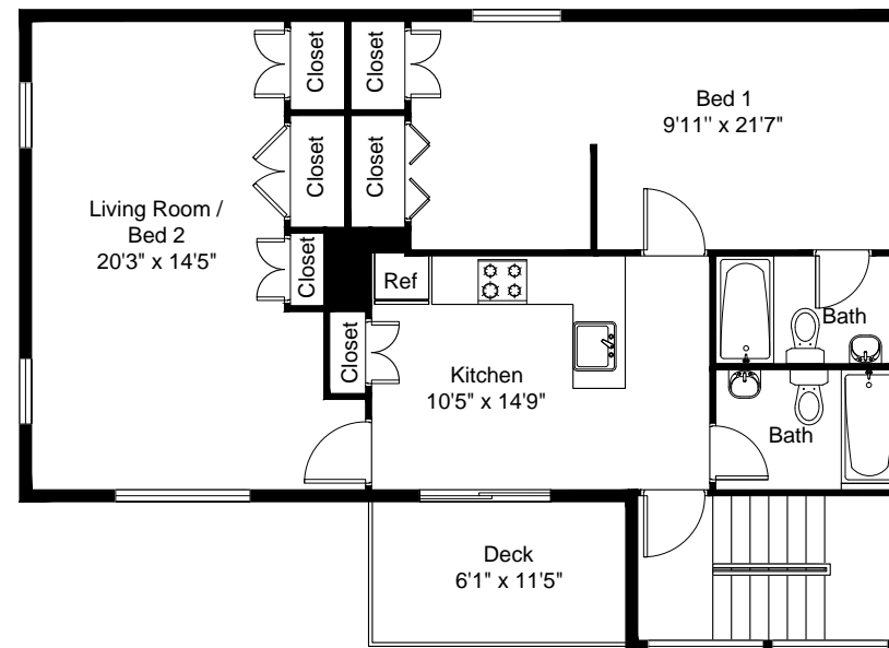
UPPER LEVEL
